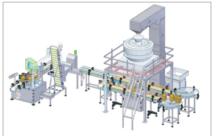
Jar Filling Line with Multihead weigher
