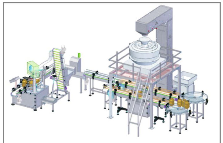
Jar Filling Line with Multihead weigher
