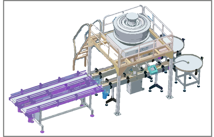
Double Track Filling Line
